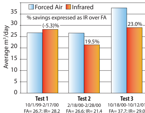
Forced Air vs. Infrared Energy Usage.
